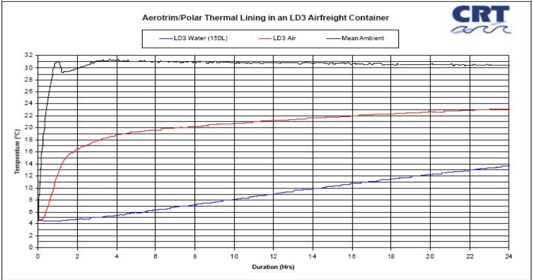
Figure 8 - Ref7: Graph of LD3 Liner Temperatures
